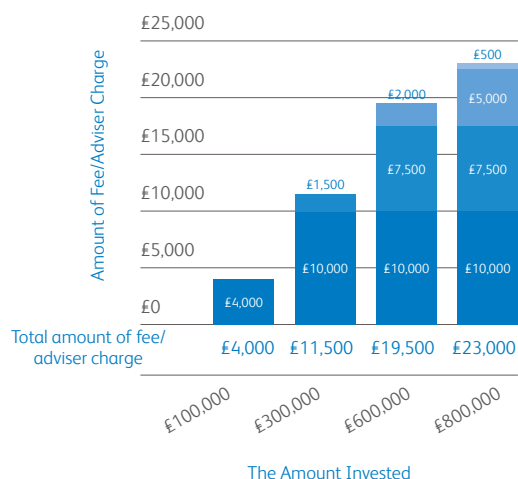
What you will pay based on an example of maximum fees for Advice and Implementation
